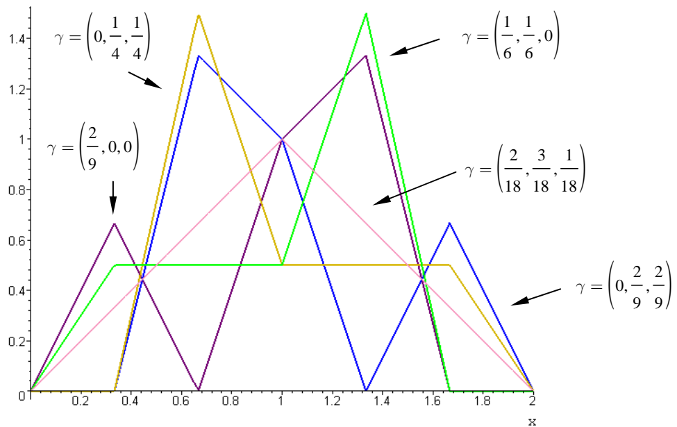
Fig. 1: densities \tilde{f}_2(3; \gamma; x)
