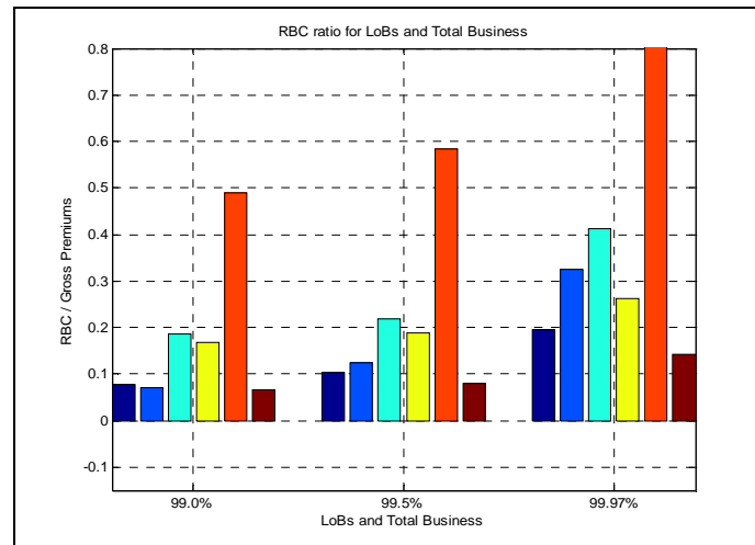
Figure 6: Company OMEGA – RBC ratio for LoBs and Total Business in case of independence for different confidence levels (Number of simulations = 1.000.000)
