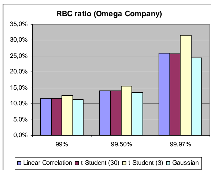
Figure 18: RBC ratio (OMEGA Company) under different dependence assumptions (Elliptical Copulas and Linear Correlation)
