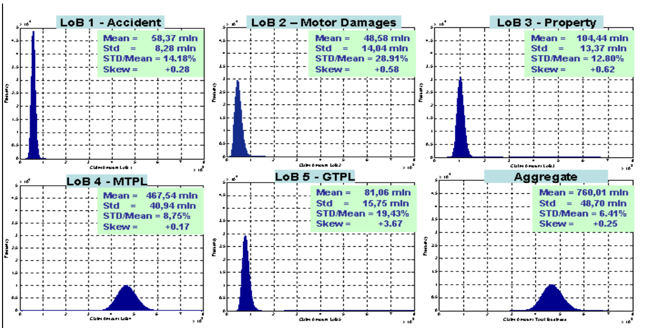
Figure 4: Company OMEGA - Simulated distributions of the Total Claim Amount for each LoB and of the Aggregate Claim Amount in case of independence (Number of simulations = 1.000.000)
