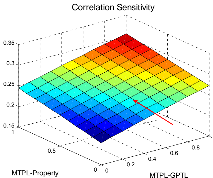
Figure 22: RBC ratio (99,5% EPSILON Company) with correlation coefficient sensitivity
