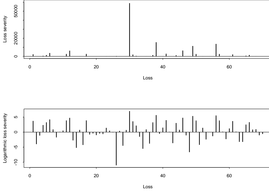
Figure 1: 70 loss severities (upper panel) and their corresponding logarithmic values centered around 0 (lower panel), sampled from a \text{LN}(\mu_{\text{int}} = 4, \sigma_{\text{int}} = 4) distribution.
