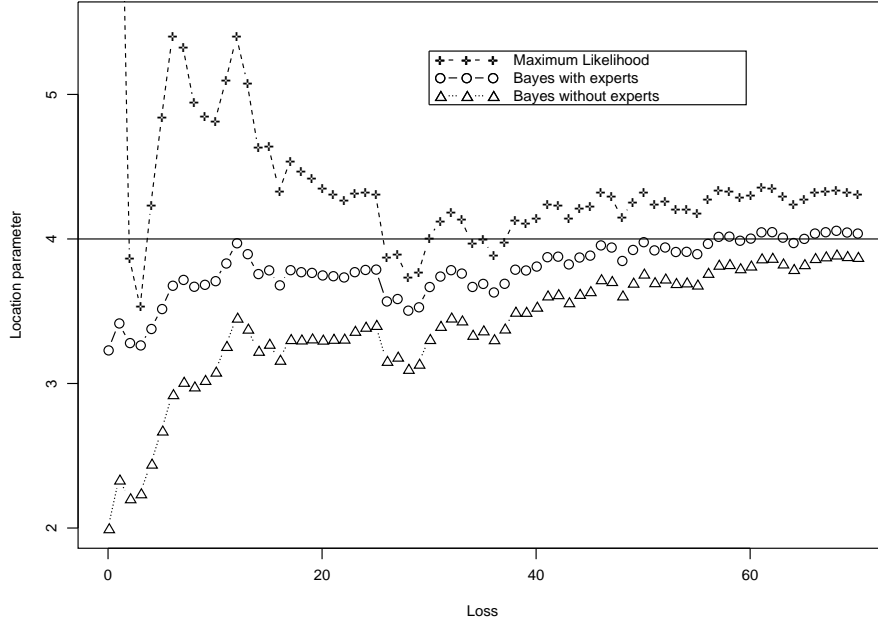
Figure 2: The Bayes estimator \hat{\mu}_k including expert opinion ( \circ ) is compared to the Bayes estimator \hat{\mu}_k^{SW} without expert opinion ( \Delta ) and to the maximum likelihood estimator \hat{\mu}_k^{MLE} ( + ). The straight line stands for the true company specific parameter \mu_{\text{int}} = 4 .
